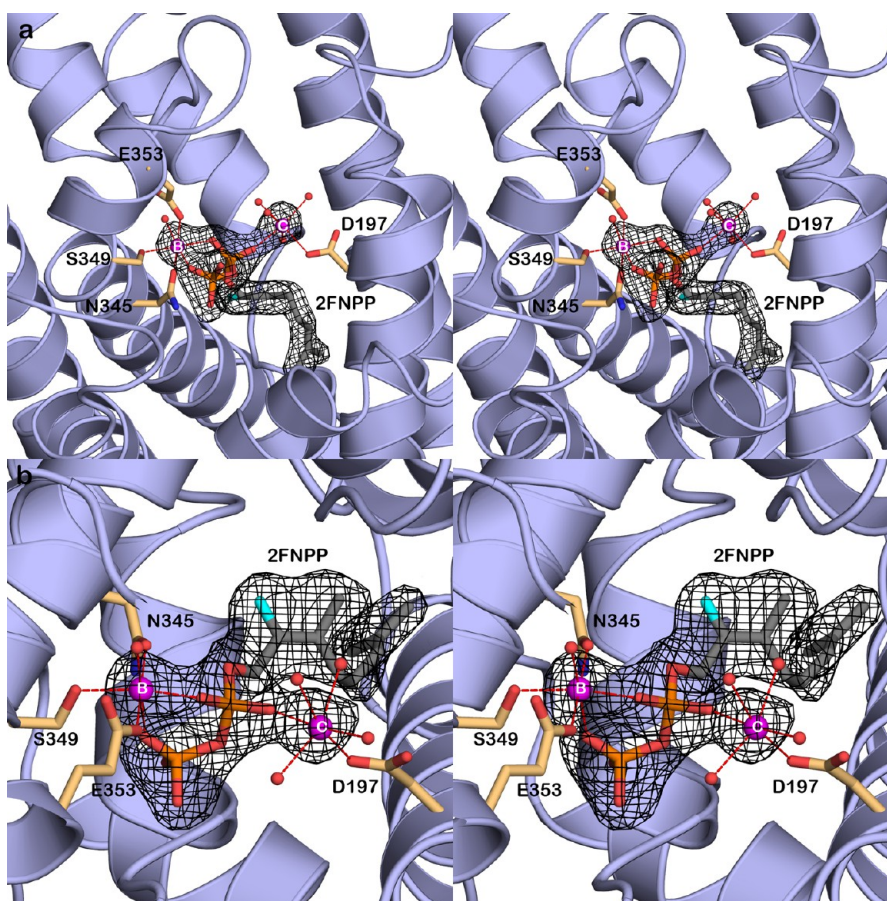
Figure 3. (a) Simulated annealing omit map of 2FNPP (contoured at 4.0\sigma ) in the MIBS-Mg 2+ 2 -2FNPP complex prepared by cocrystallization of MIBS with 2FLPP. Atoms are color-coded as follows: C = tan (protein) or gray (2FNPP), O = red, N = blue, P = orange, F = cerulean blue, Mg 2+ ions = magenta spheres, solvent molecules = red spheres. Metal coordination interactions are shown as red dotted lines. (b) Same map as (a), but rotated by ca. 90° and zoomed in to show the cis -isoprenoid linkage of 2FNPP.
