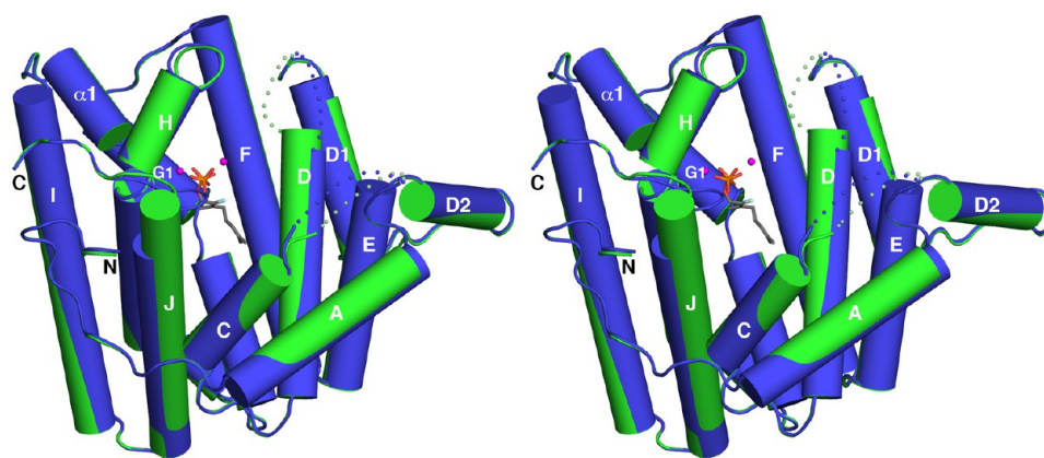
Figure 2. Superposition of unliganded MIBS (green) with the MIBS-Mg 2+ 2 -2FGPP complex (blue, PDB ID: 3V1X); 2FGPP appears as a stick figure and Mg 2+ ions are spheres. Dotted lines indicate disordered polypeptide segments. The A–C loop and the D–D1 loop remain disordered in the liganded enzyme, indicating that the enzyme active site in the MIBS–Mg 2+ 2 -2FGPP complex remains in a partially open conformation.
