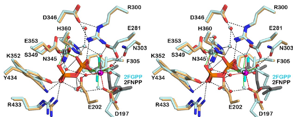
Figure 4. Superposition of the MIBS- \text{Mg}^{2+} -2FNPP complex (color-coded as in Figure 3) and the MIBS- \text{Mg}^{2+} -2FGPP complex (all atoms pale cyan) reveals alternative conformations for the isoprenoid tails of the configurational isomers. Metal coordination and hydrogen bond interactions are shown as red and black dotted lines, respectively.
