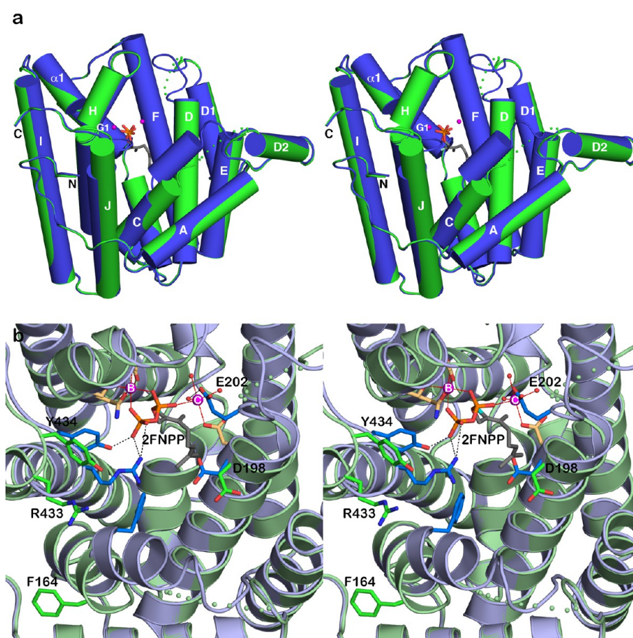
Figure 5. (a) Superposition of the MIBS- \text{Mg}^{2+} -2FNPP complex (blue) and unliganded MIBS (green) reveals conformational changes that occur upon ligand binding. These conformational changes are more extensive than those observed upon the binding of 2FGPP (compare with Figure 2), including the ordering of the A-C loop, helix C (note the significant movement of F164), the D-D1 loop, and the N-terminus of helix J. (b) Close-up view of the superposition of the MIBS- \text{Mg}^{2+} -2FNPP complex (light blue ribbon, side chains with blue or tan carbon atoms) and unliganded MIBS (light green ribbon, side chains with green carbon atoms) reveals induced-fit conformational changes that accompany the binding of 2FNPP, \text{Mg}^{2+}_B , and \text{Mg}^{2+}_C . The active site remains partially open in the MIBS- \text{Mg}^{2+} -2FNPP complex; in the fully closed conformation, a hydrogen bonded salt link is expected to form between R433 and D198, which in the partially open active site conformation are separated by more than 5 Å.
