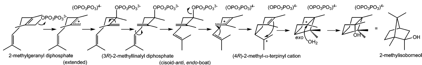
Figure 1. Proposed cyclization mechanism of MIBS.
